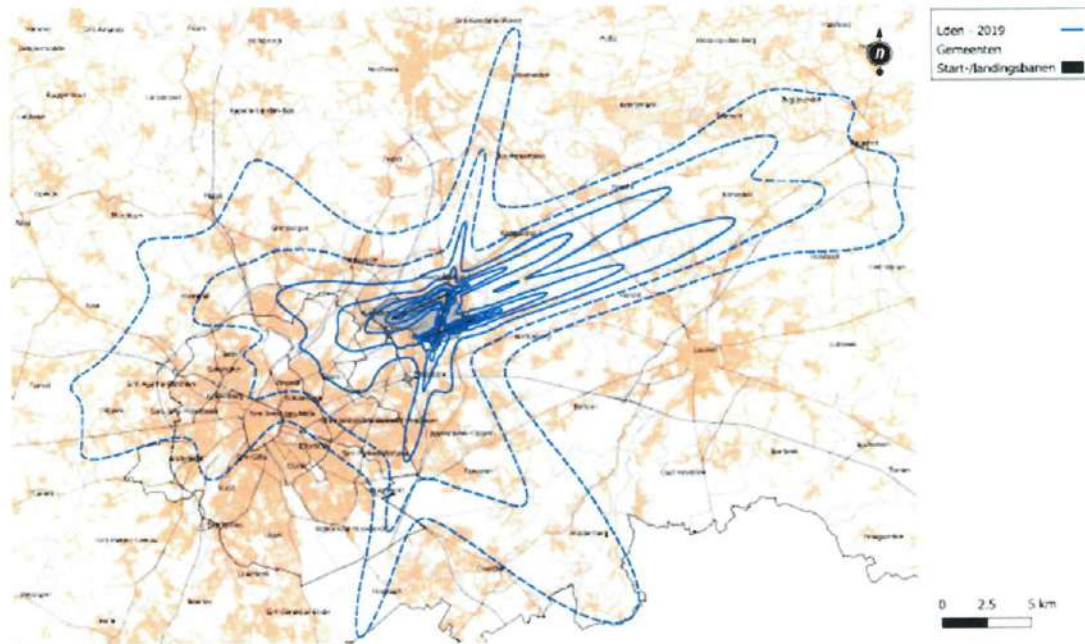
Figuur 6-29: contouren 70 dB(A) (5x, 10x, 20x, 50x, 100x) – 2019 – dag (07u-23u)
